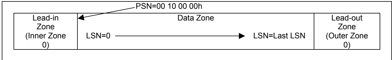
Figure 60 — Layout of Single Layer BD-ROM Information Zone
