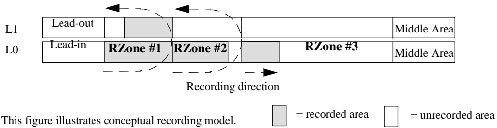
Figure 40 — Example of Layer Jump Recording
