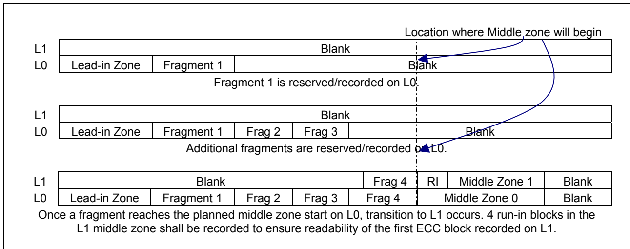
Figure 57 — Example: Crossing the Layers During Recording
