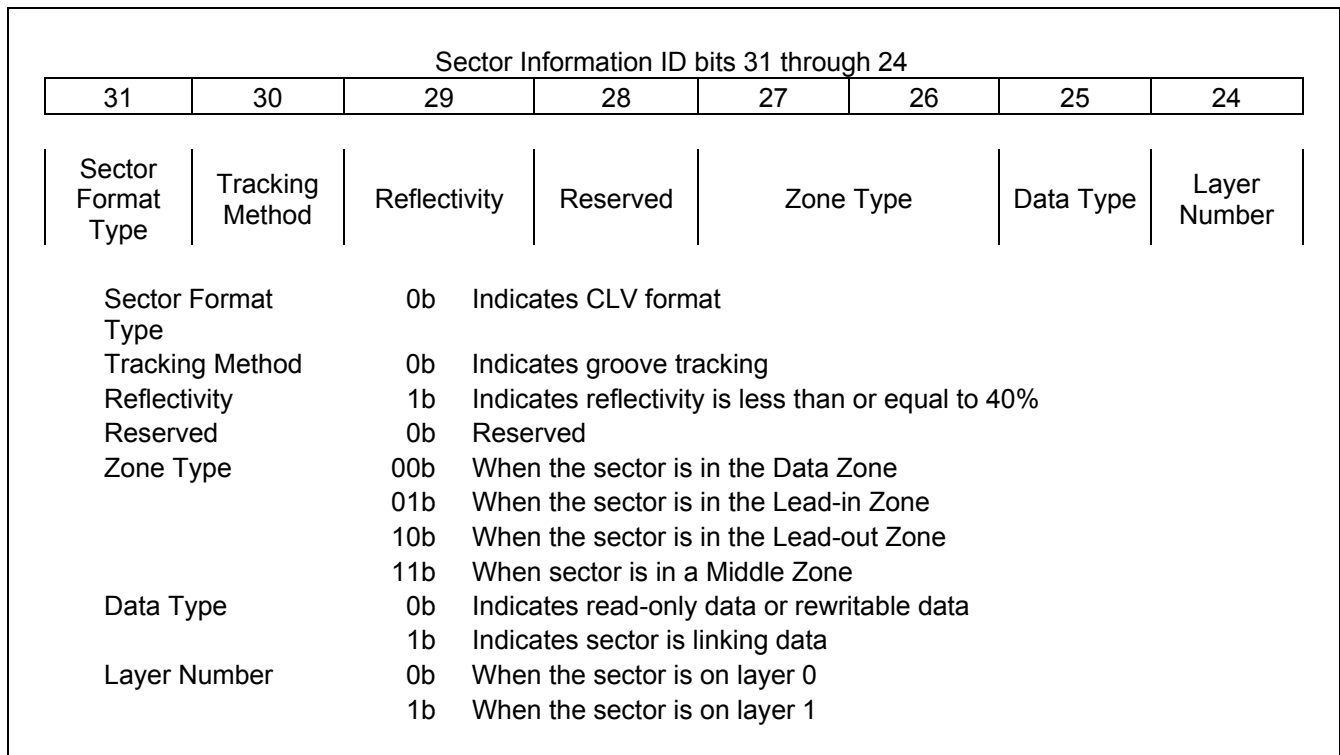
Figure 36 — DVD-R DL ID field Sector Information details
