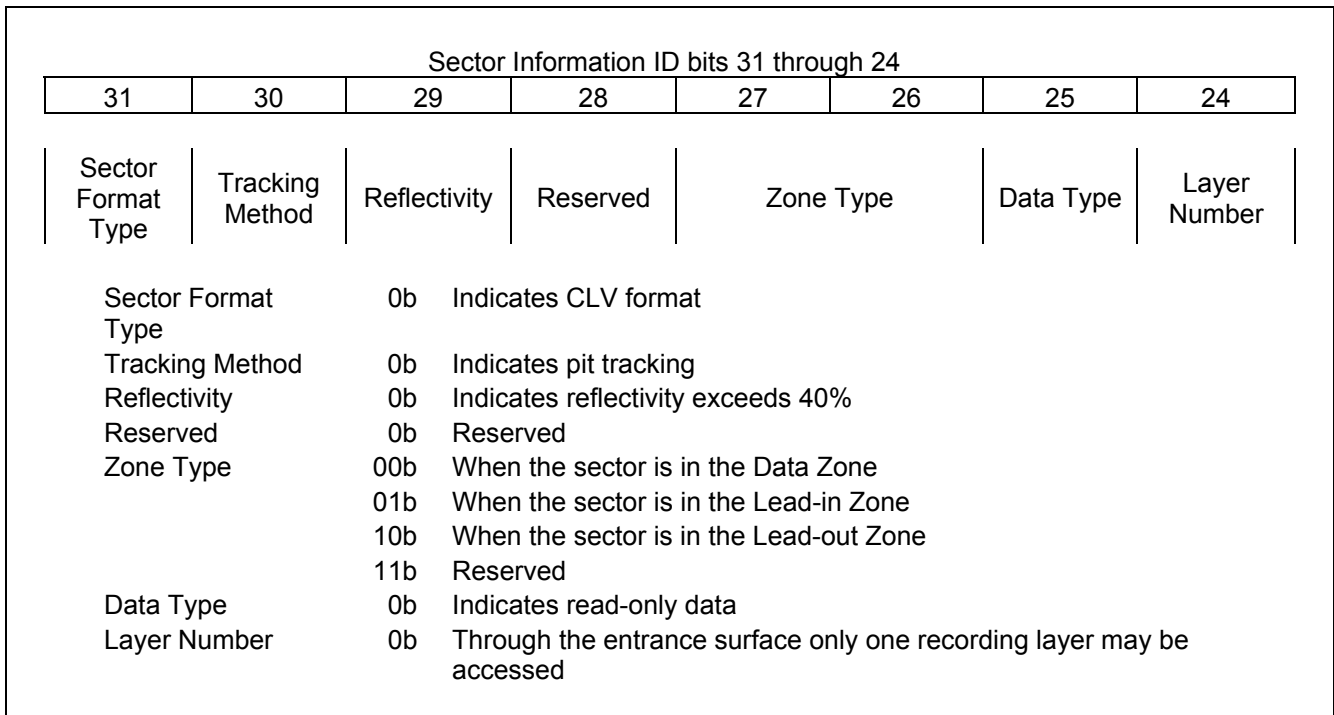
Figure 48 — DVD+R ID field Sector Information details
