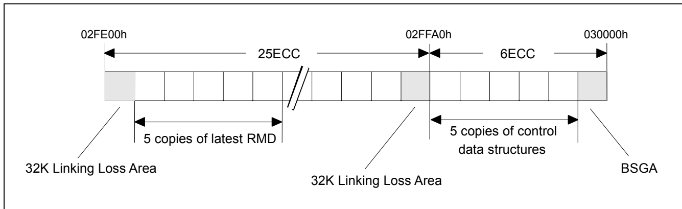
Figure 33 — Structure of Extra Border Zone
