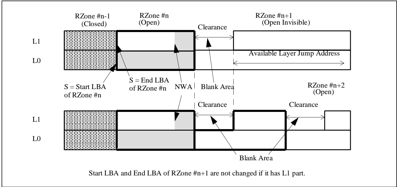
Figure 38 — Blank Areas and RZone Shape
