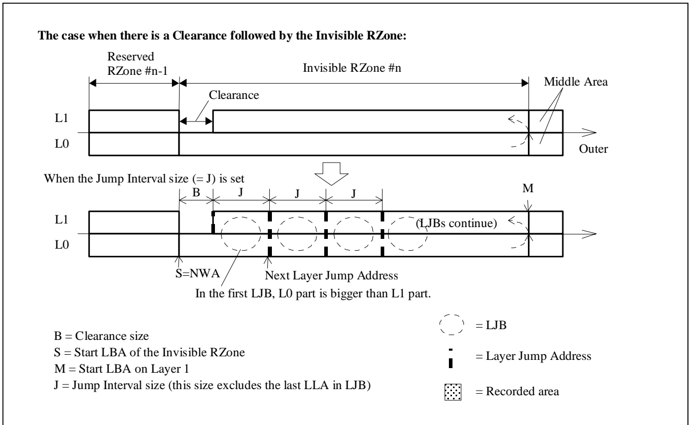
Figure 42 — Regular Interval Layer Jump
