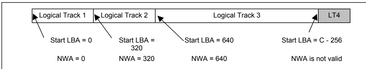
Figure 81 — Status after Splitting Logical Track 2
