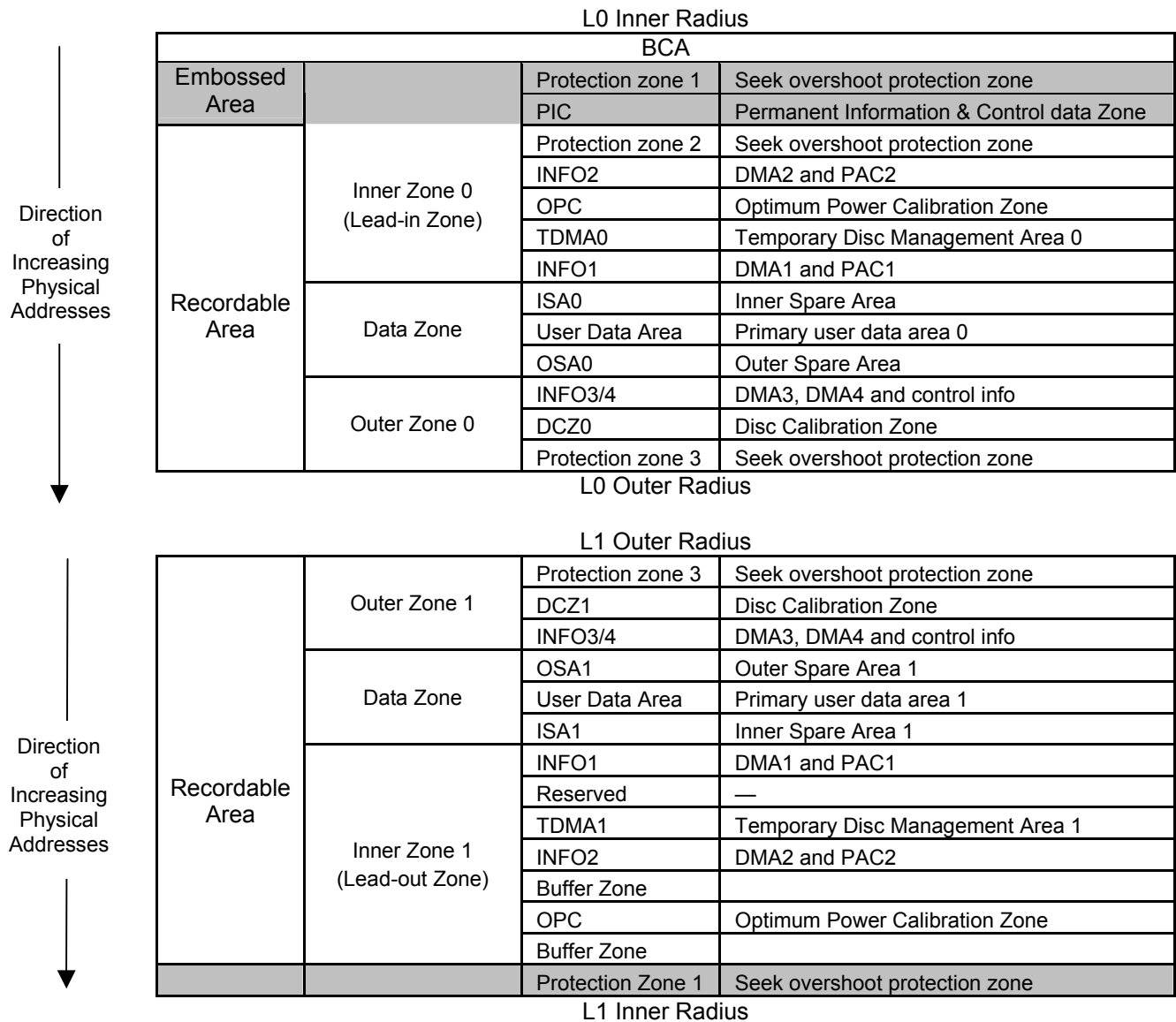
Figure 65 — BD-R Information Zones
