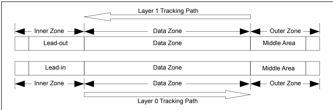
Figure 5 — General Dual Layer OTP Structure
