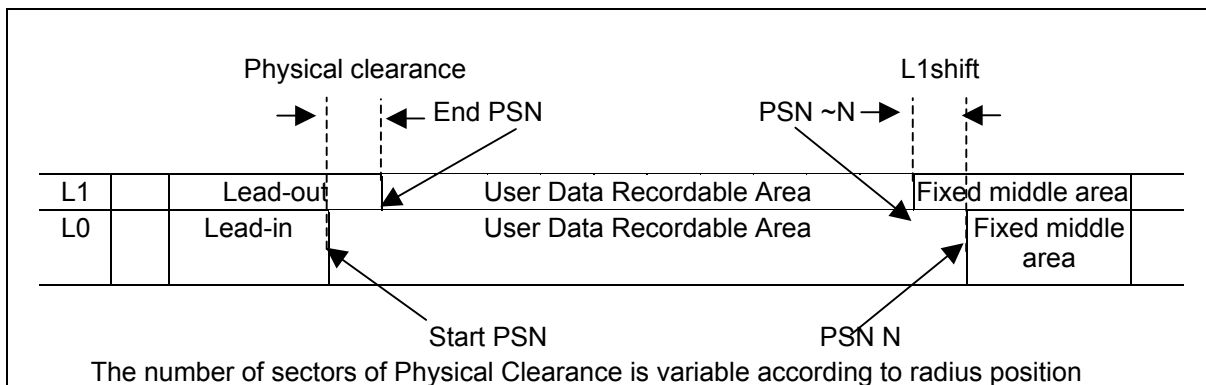
Figure 35 — Physical Overview of Layers
