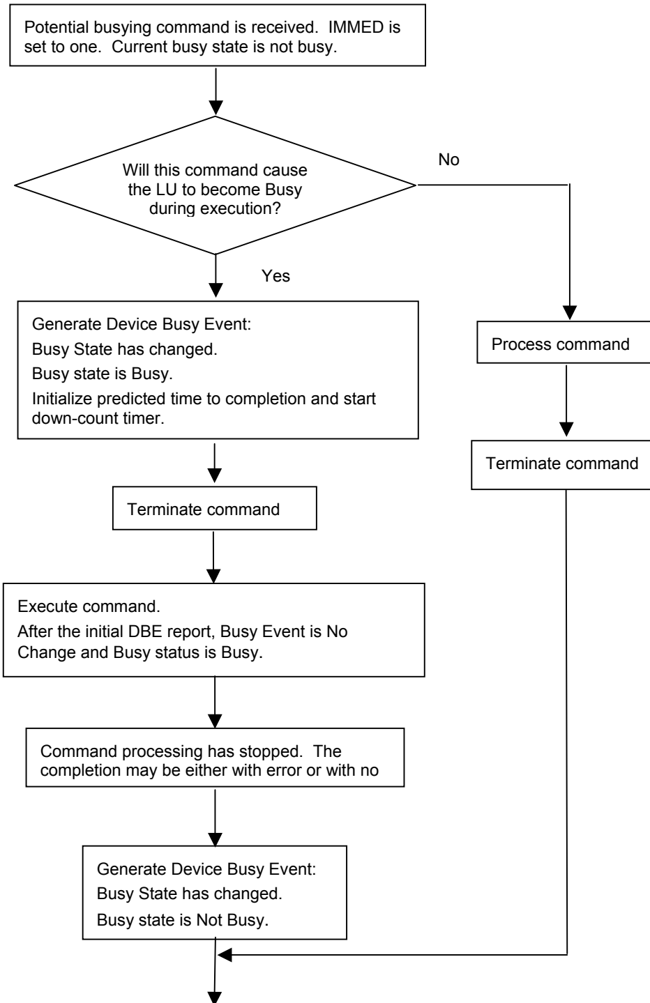
Figure 126 — Execution of a command that may cause Drive Busy
