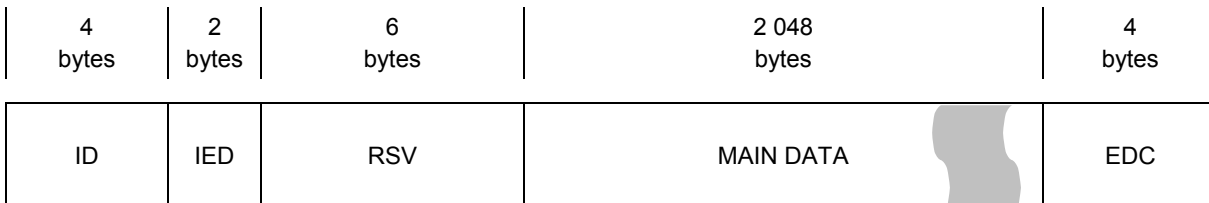
Figure 67 — Logical Layout of a HD DVD Data Sector
