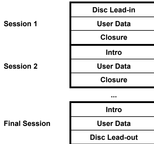
Figure 45 — General Layout of a Multi-Session DVD+R
