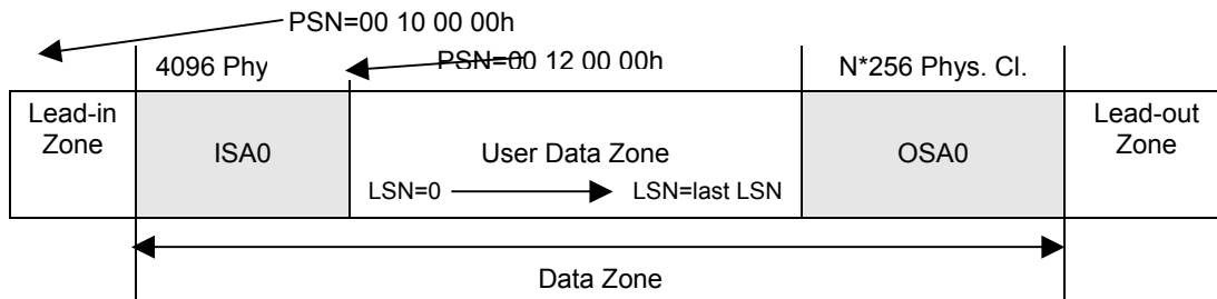
Figure 105 — Layout of Single Layer BD-RE Disc
