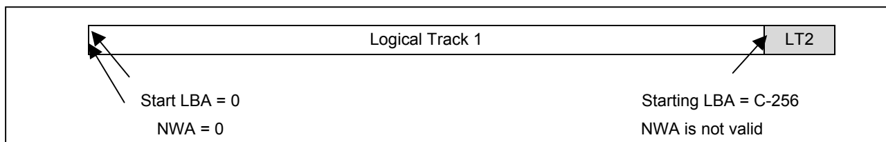
Figure 95 — Create, Write, and Close Small Outer Logical Track
