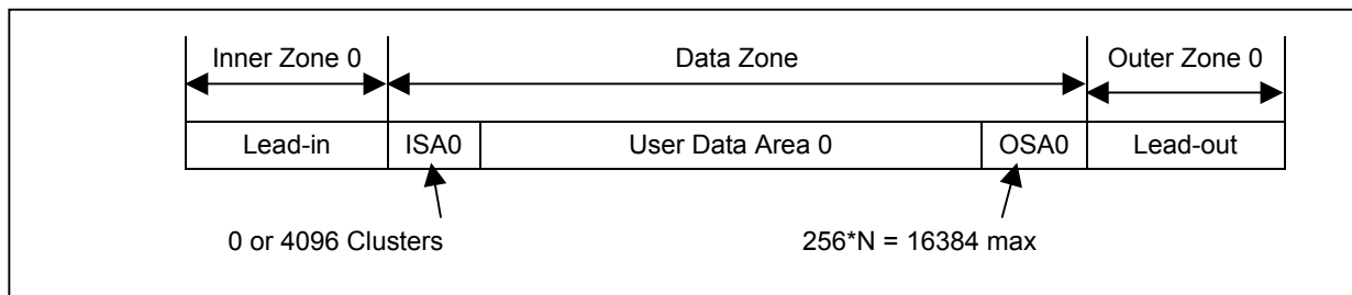
Figure 82 — SL BD-R Information Zone
