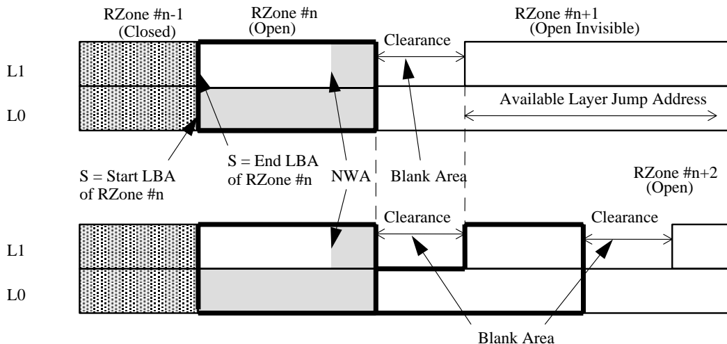
Figure 37 — Blank Areas and RZone Shape
