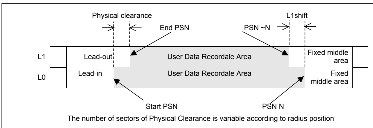
Figure 34 — Physical Overview of Layers
