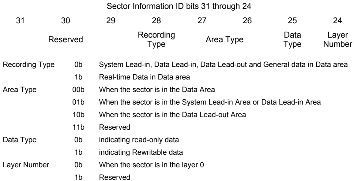
Figure 74 — ID Field for HD DVD-RAM
