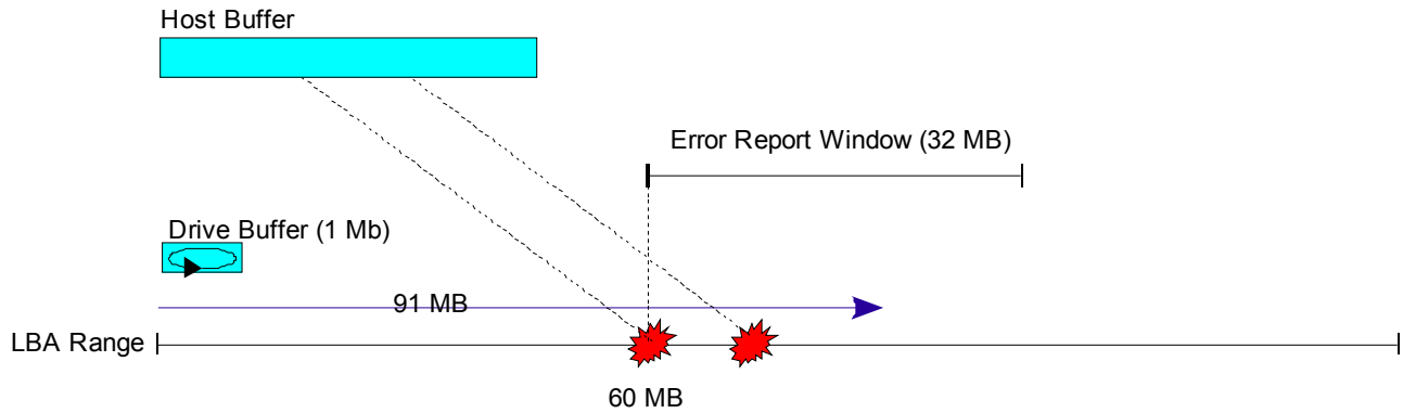
Figure 119 — Last Chance to Notify Host of Defects
