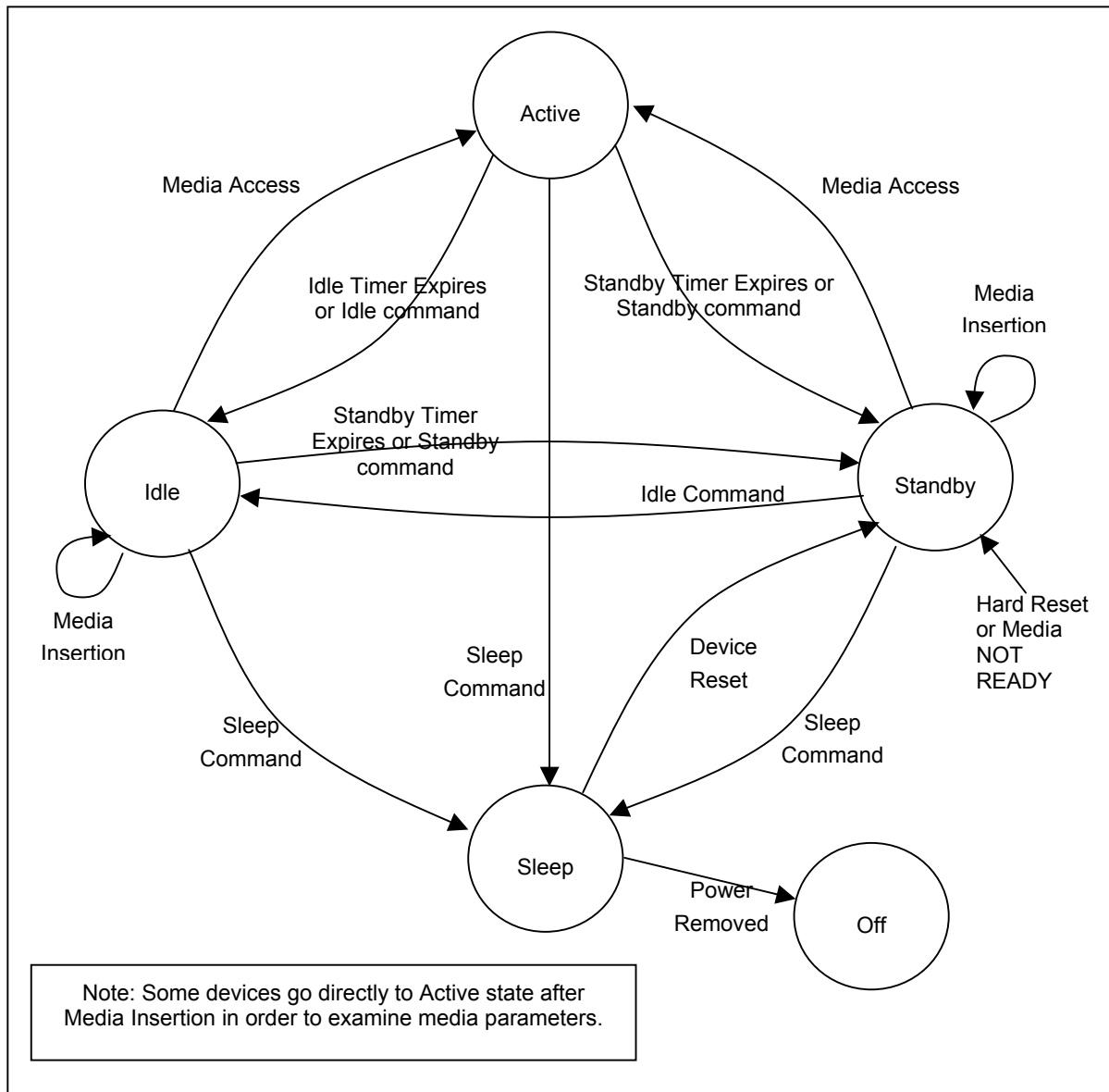
Figure I.1 — Power Management STATE Diagram
