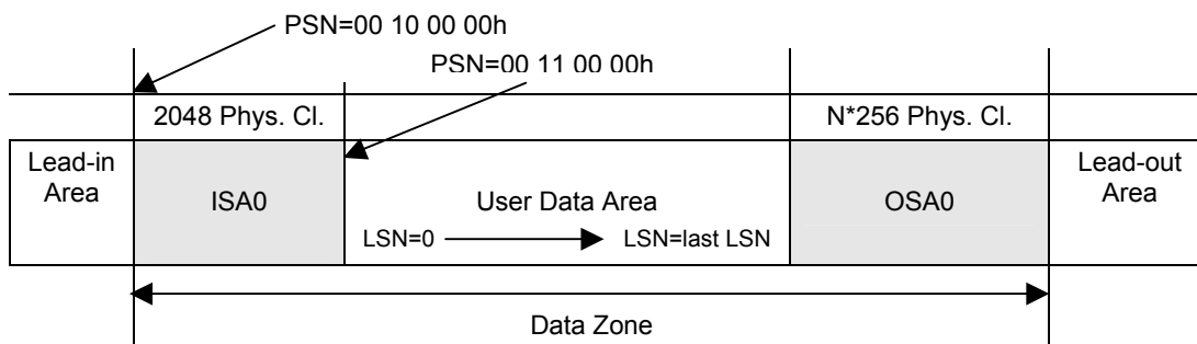
Figure 102 — Layout of Single Layer BD Disc
