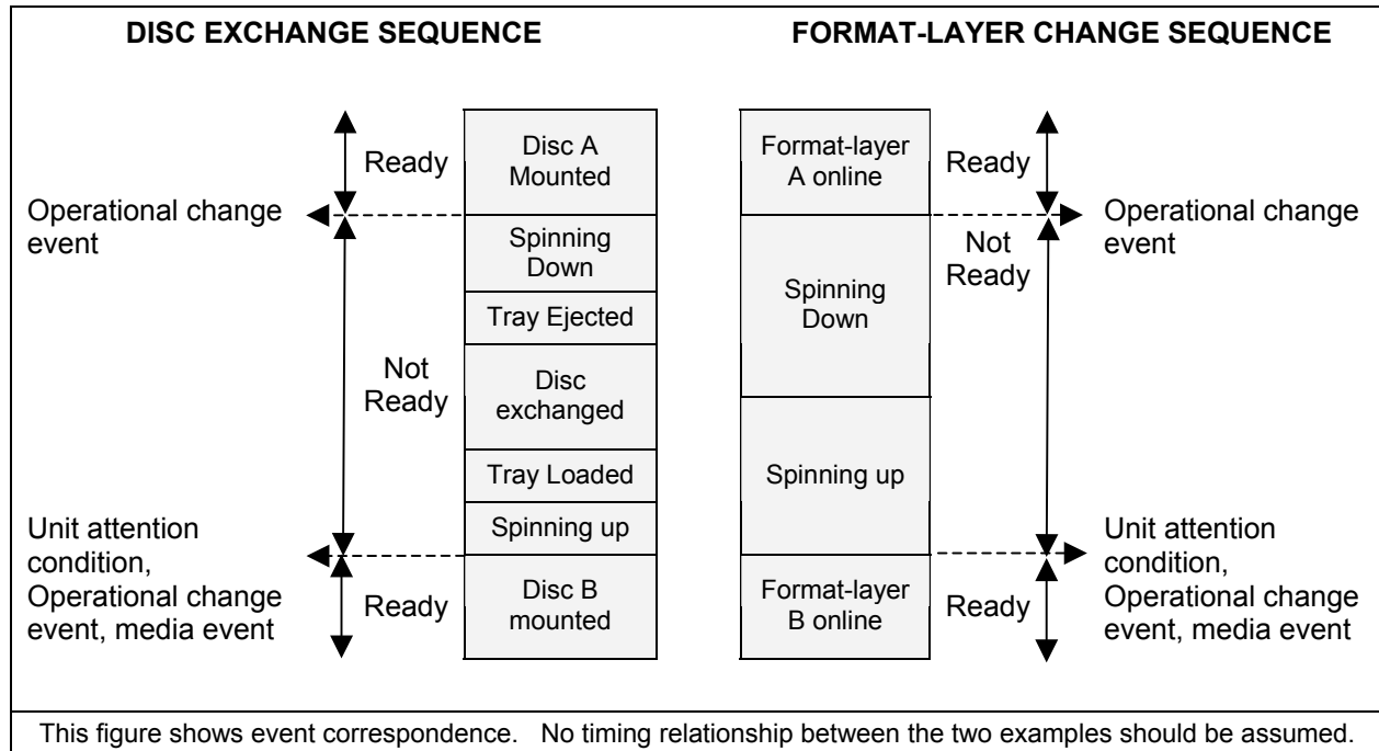
Figure 124 — Comparison of disc exchange and Format-layer change
