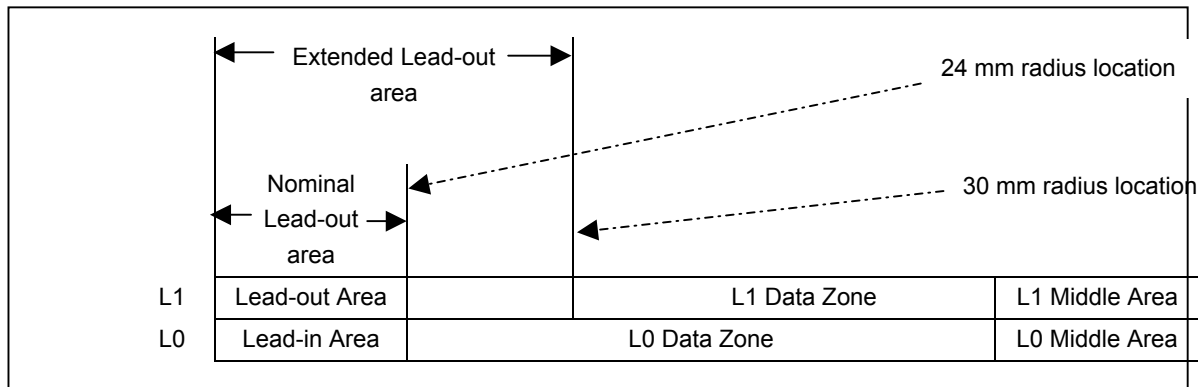
Figure 54 — Finalization Areas on DVD+R DL
