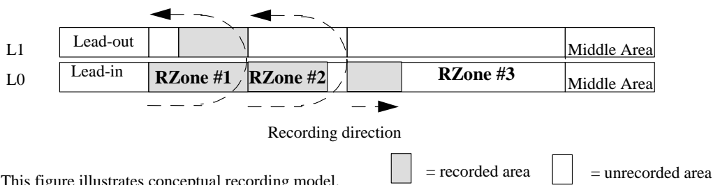
Figure 39 — Example of Layer Jump Recording
