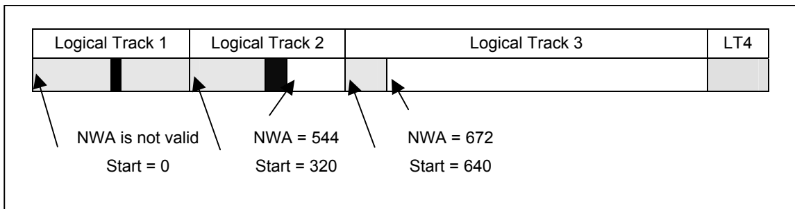
Figure 101 — Status after LOW of LBA 256
