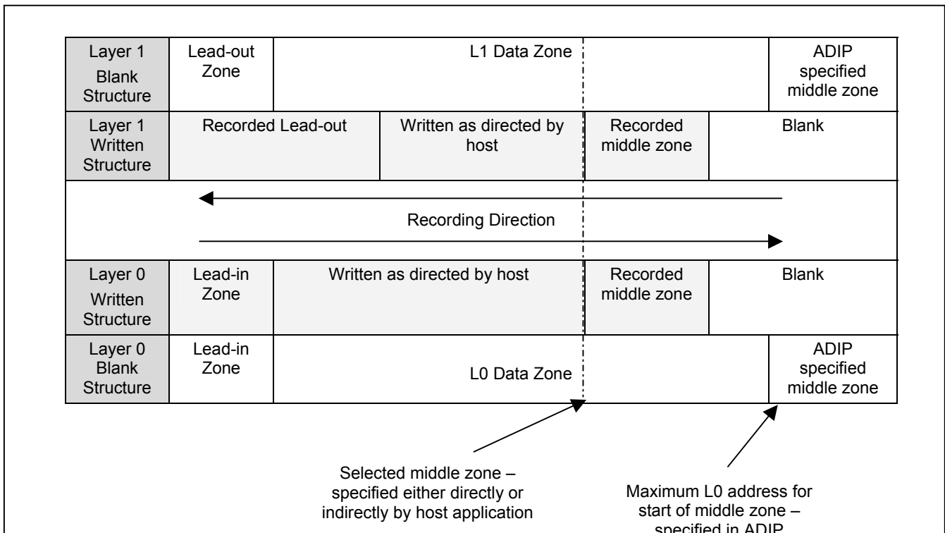
Figure 49 — Blank and Recorded Structure of a DVD+R DL Disc
