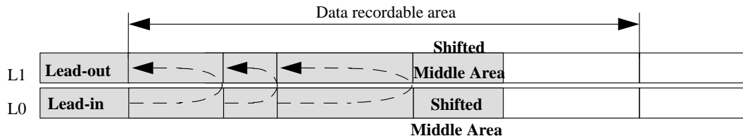
Figure 43 — Disc Final Closure in Layer Jump Recording Mode
