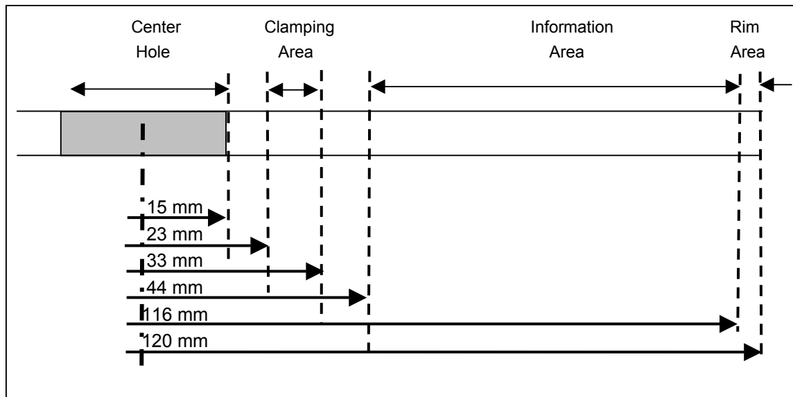
Figure 66 — The Areas of a HD DVD Medium
