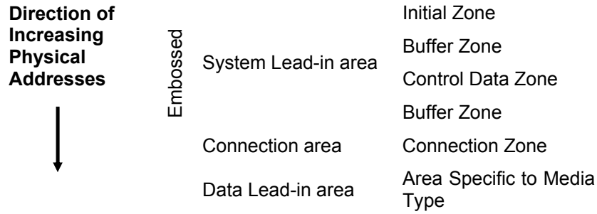
Figure 70 — General Layout of Lead-in area
