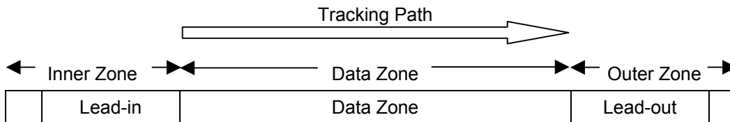
Figure 3 — General Single Layer Structure
