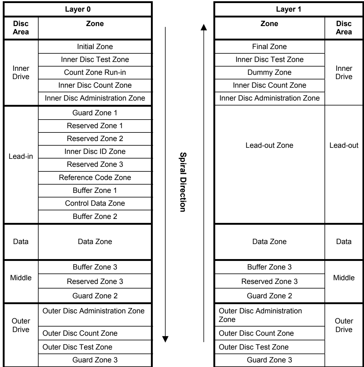
Figure 57 — Logical Layout of a DVD+RW DL Disc
