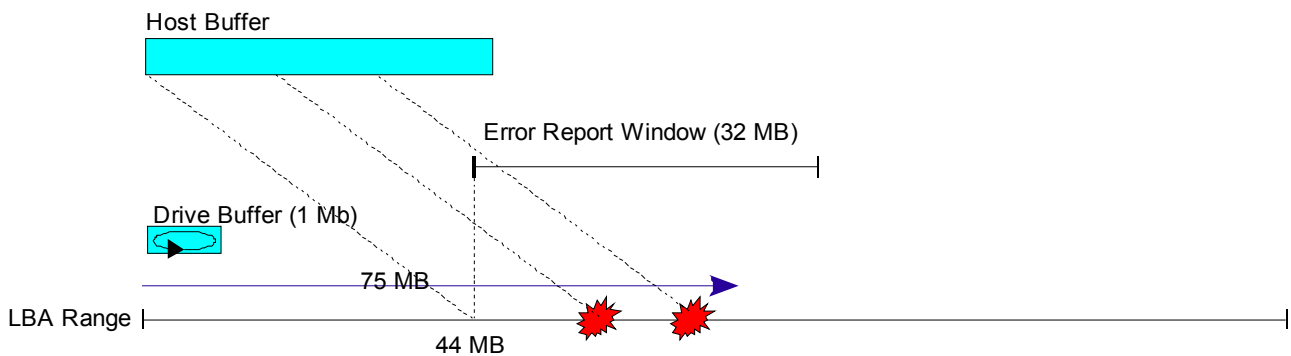
Figure 118 — Defects appear in the Error Report Window
