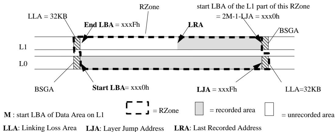
Figure 36 — RZone structure for Layer Jump recording
