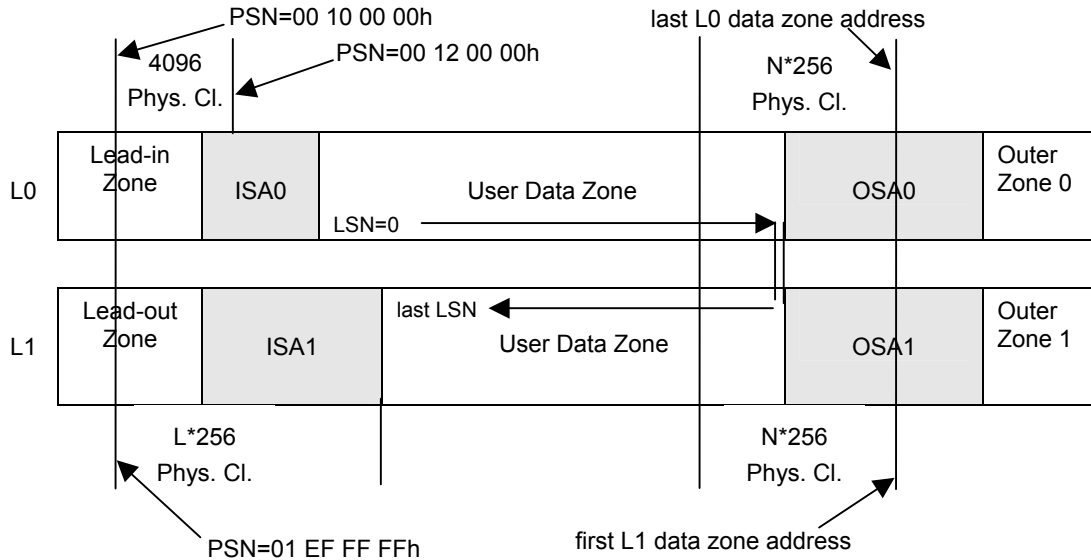
Figure 106 — Layout of Dual Layer BD-RE Disc
