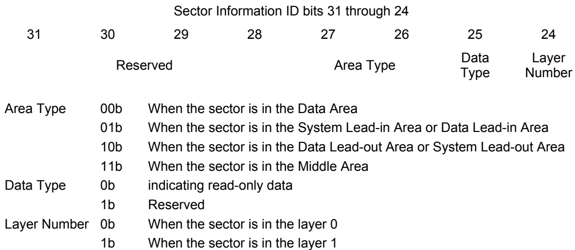
Figure 71 — ID Field for HD DVD-ROM
