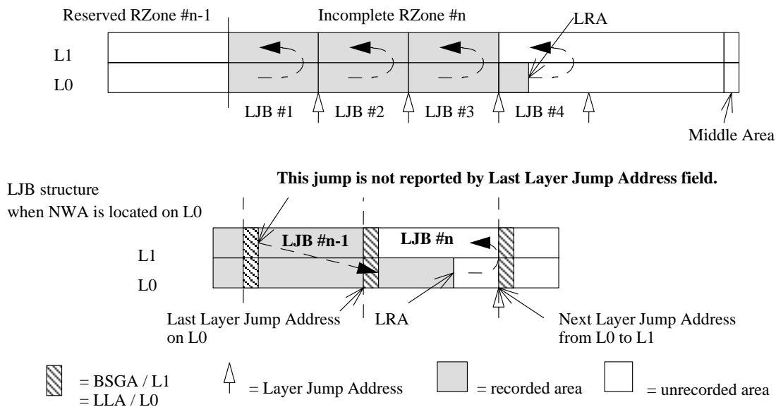
Figure 40 — LJB Structure of Invisible/Incomplete RZone
