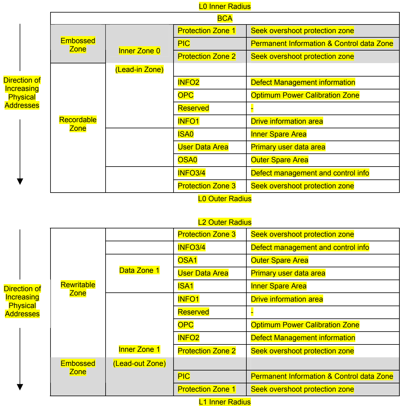
Figure 104 — BD-RE Information Zone
