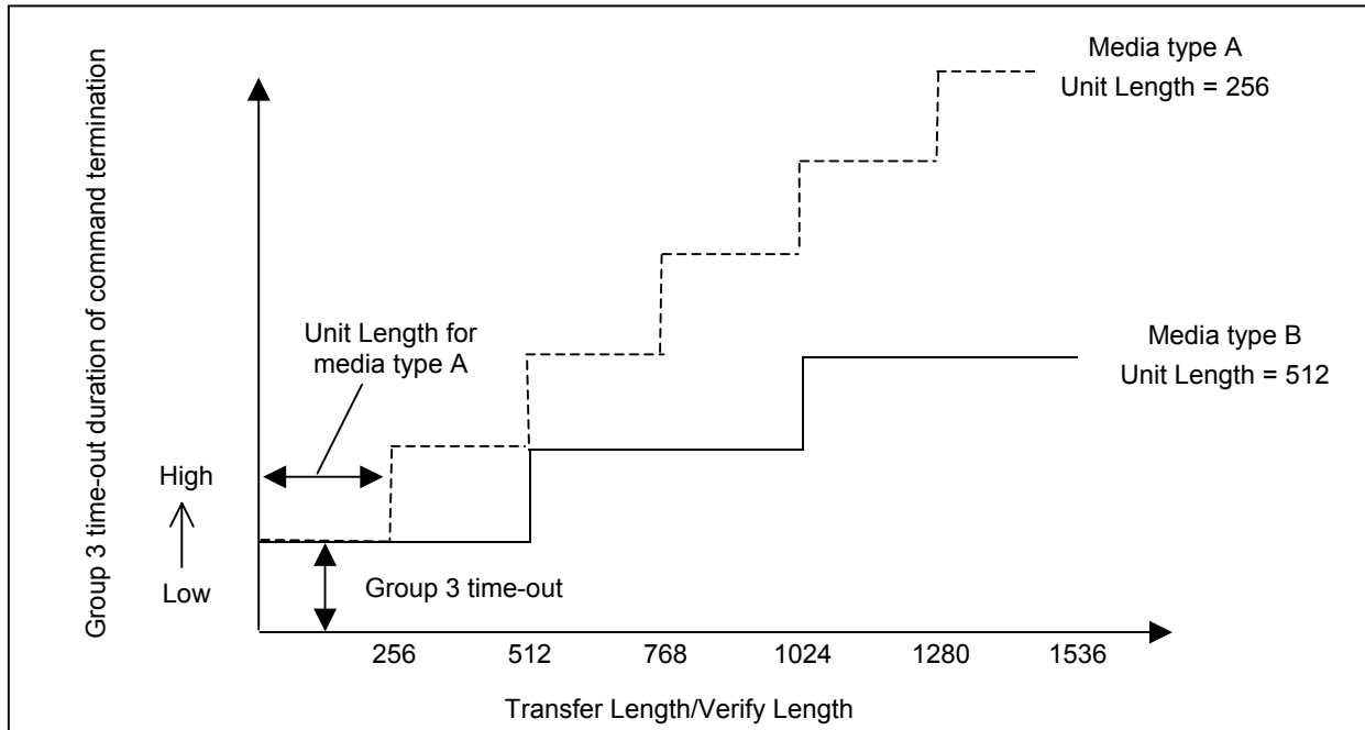
Figure 8 — Adjustment of Command Termination Time on Different Media
