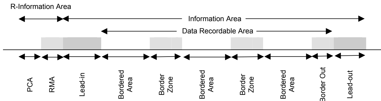
Figure 33 — Border Zone and Bordered Area
