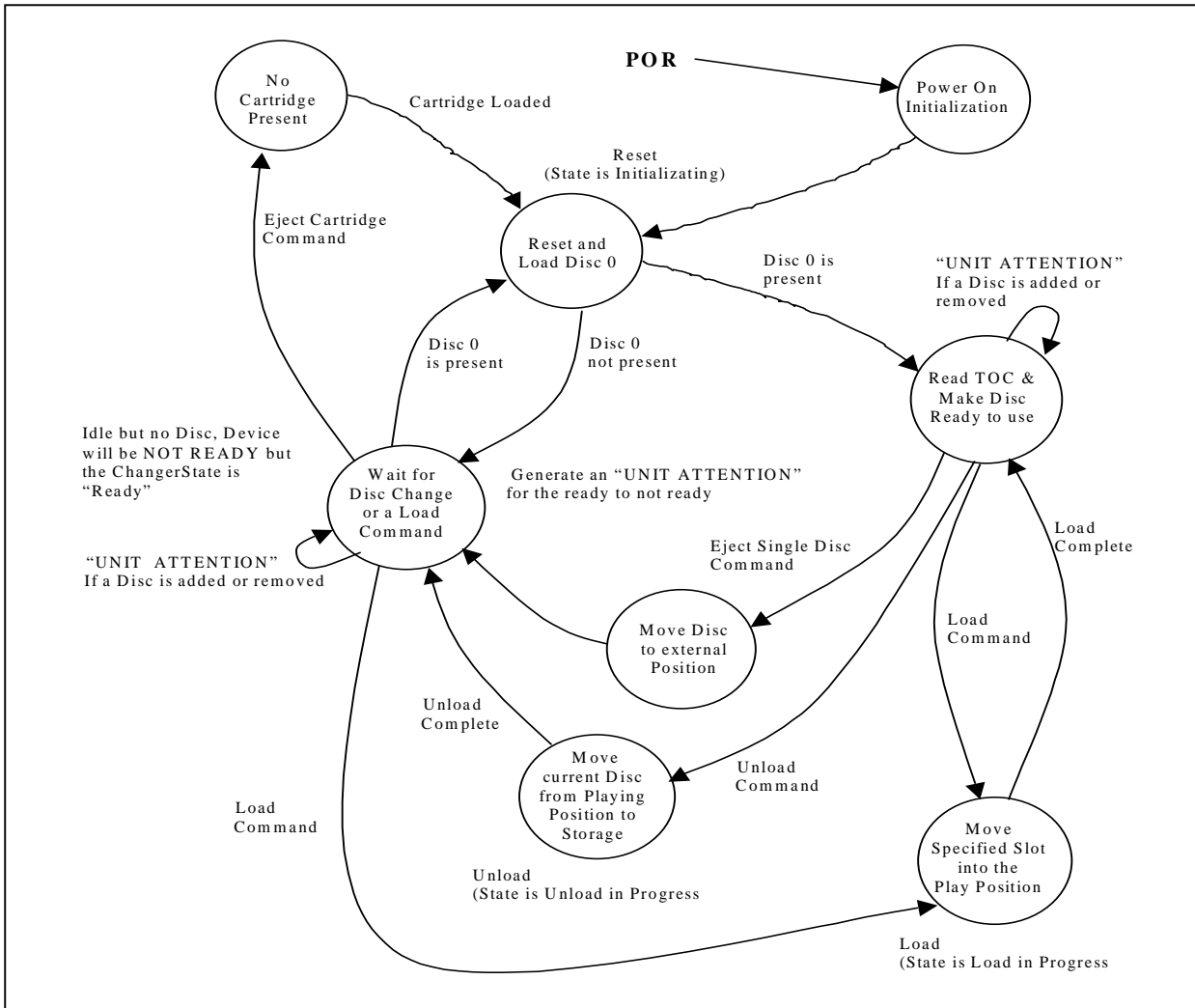
Figure 122 — Changer State Diagram
