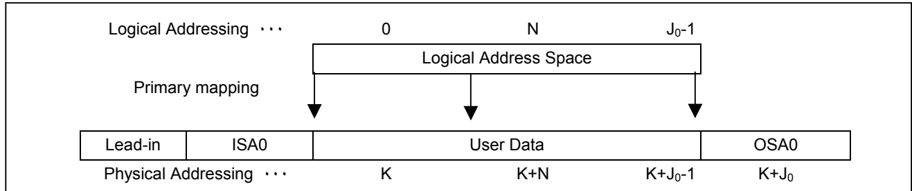
Figure 88 — Logical to Physical Addressing on Single Layer
