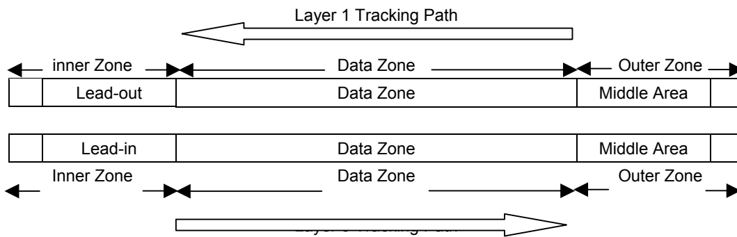
Figure 5 — General Dual Layer OTP Structure
