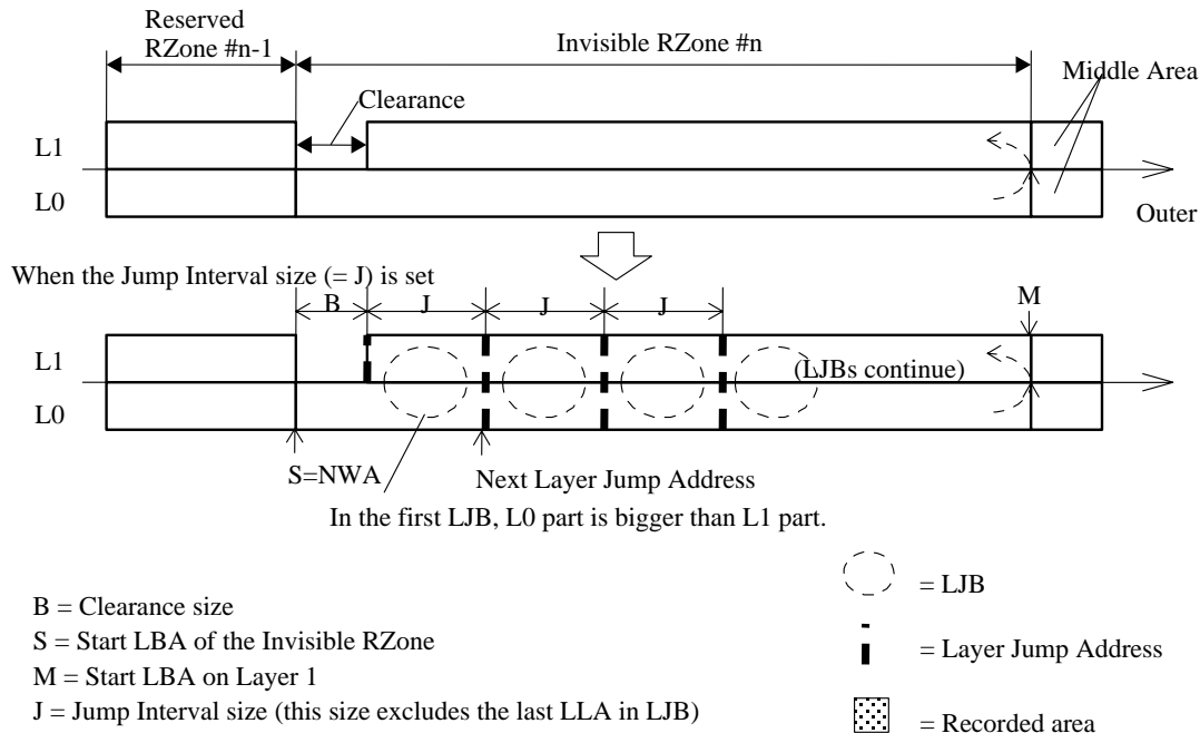
Figure 41 — Regular Interval Layer Jump
