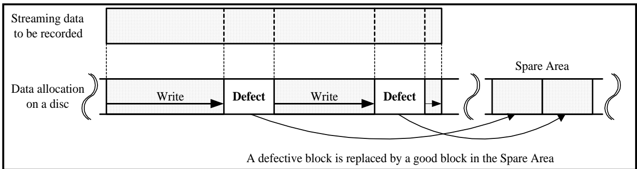
Figure 112 — Example of Data Allocation in case of Linear Replacement
