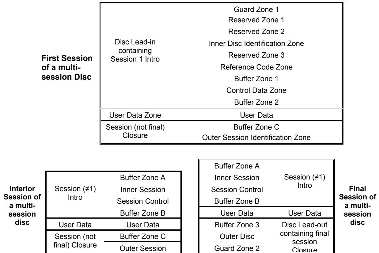
Figure 46 — Zones of a Session
