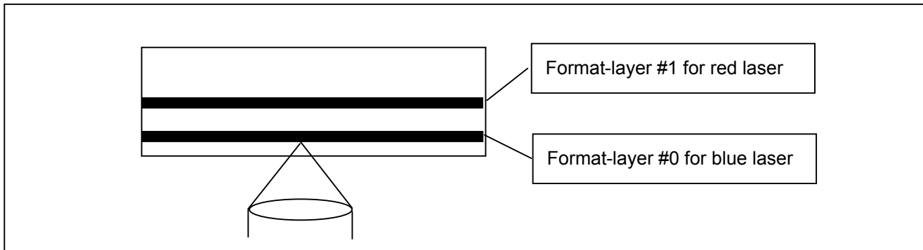
Figure 123 — Example of a Hybrid Disc
