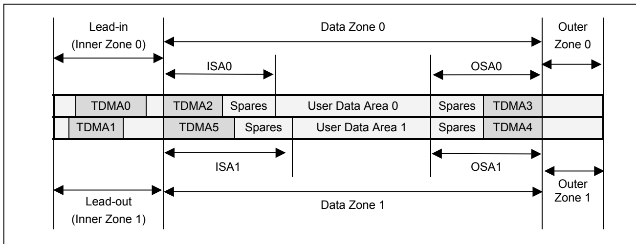
Figure 85 — TDMA Allocation on DL BD-R
