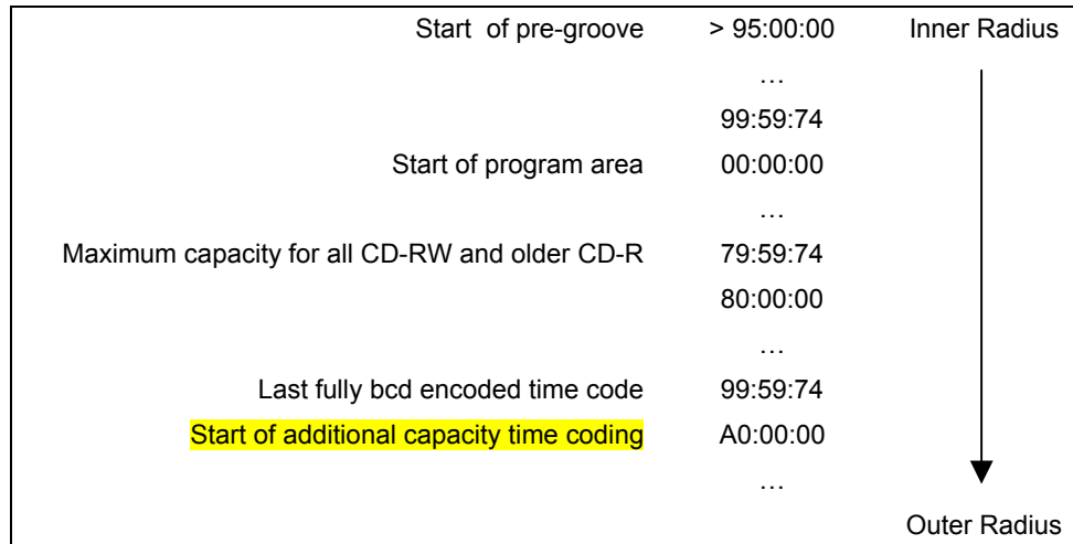
Figure 18 — Time Codes in CD-R and CD-RW Pre-groove
