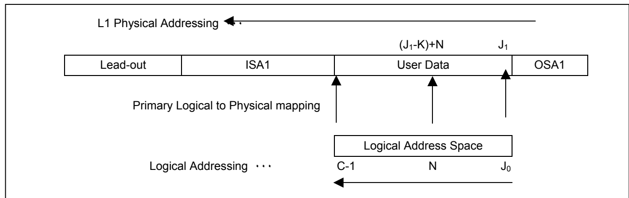
Figure 89 — Logical to Physical Addressing on Dual Layer
