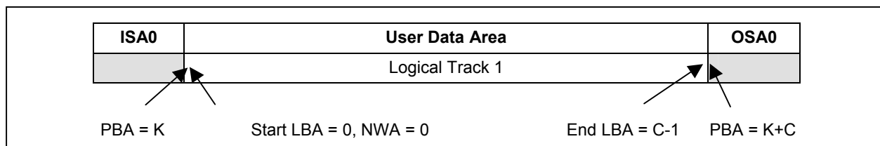
Figure 94 — Status after Formatting SRM+POW
