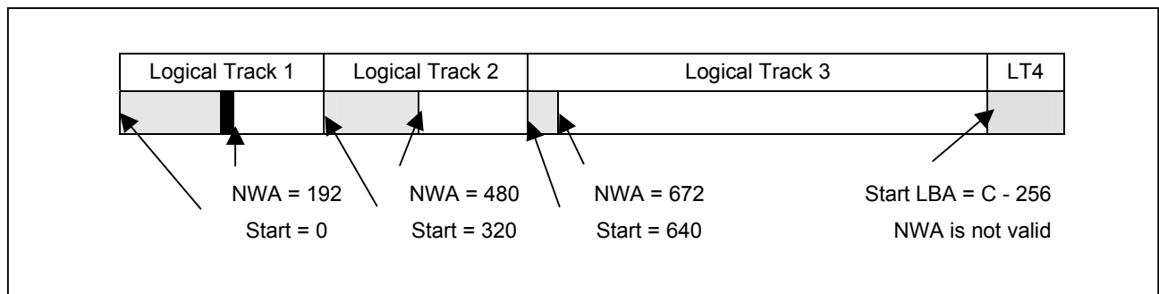
Figure 99 — Status after LOW to LBA 256
