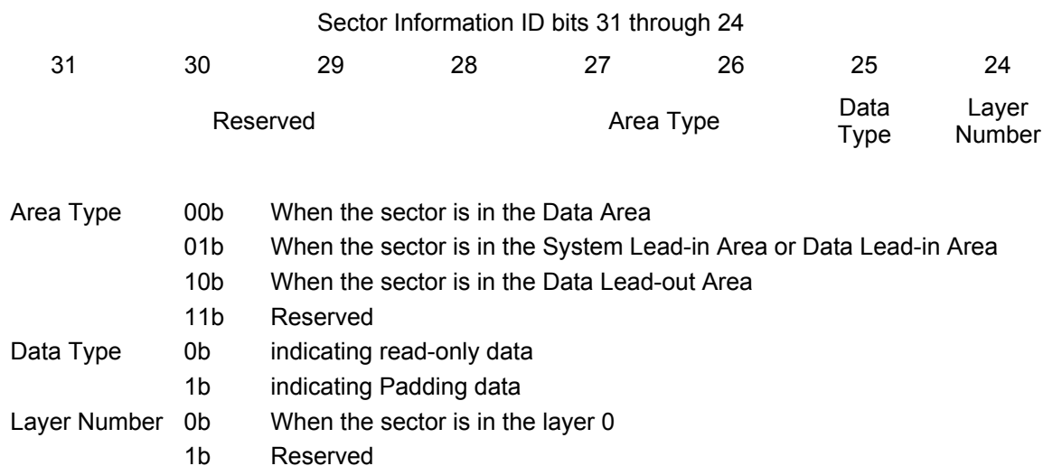
Figure 72 — ID Field for HD DVD-R
