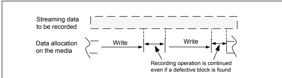
Figure 113 — An example of data allocation on the Stream recording operation
