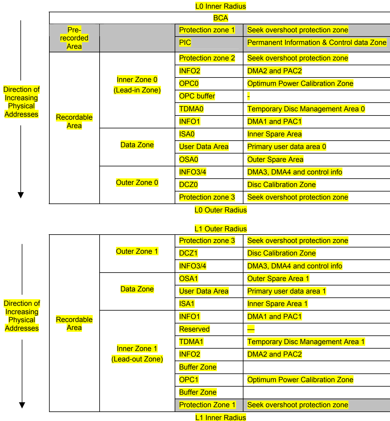
Figure 81 — BD-R Information Zones
