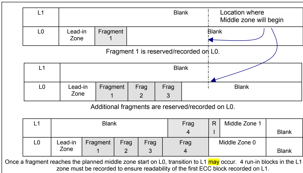
Figure 53 — Example: Crossing the Layers During Recording
