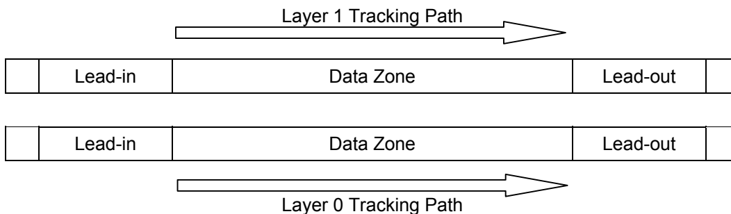
Figure 4 — General Dual Layer PTP Structure
