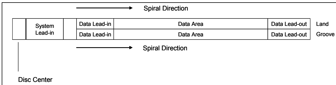
Figure 73 — Single Layer, Single Sided Disc
