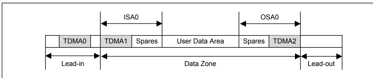
Figure 83 — TDMA Allocation on SL BD-R
