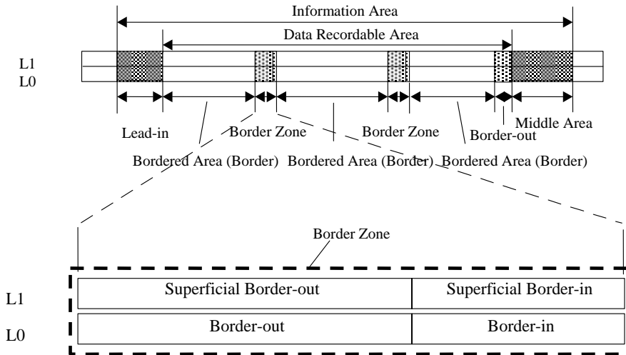
Figure 38 — Border Zone Structure for DVD-R Dual Layer media
