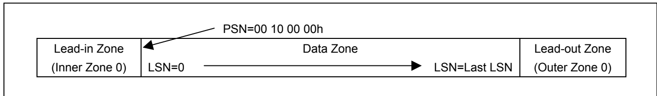
Figure 76 — Layout of Single Layer BD-ROM Information Zone
