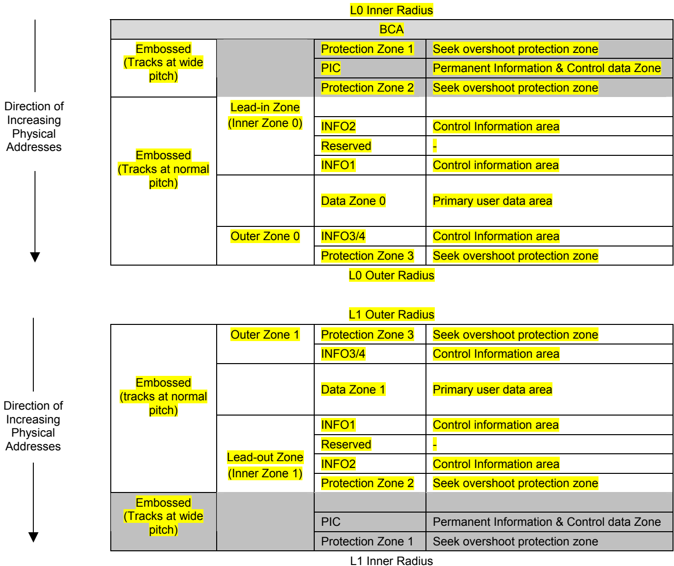
Figure 78 — BD-ROM Information Zone
