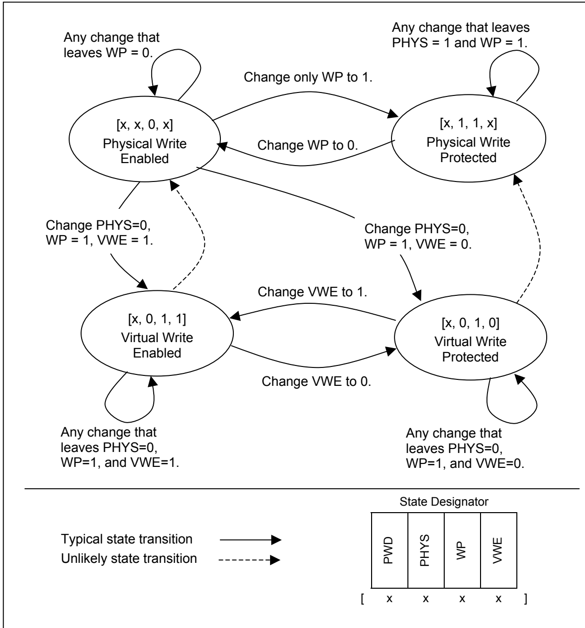
Figure 107 — Physical and Virtual Write Protect State Diagram
