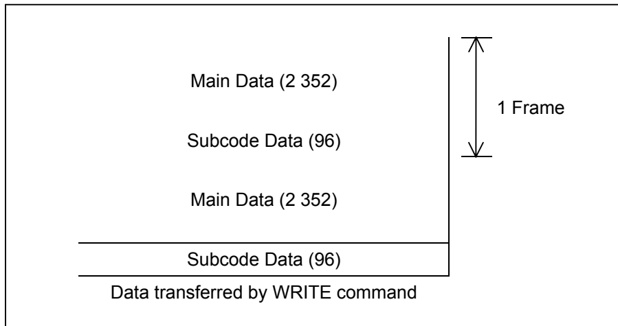
Figure 127 — Location of Sub-channel Data
