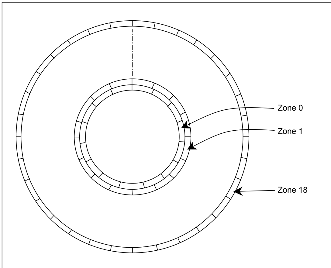
Figure 75 — HD DVD-RAM Zoning
