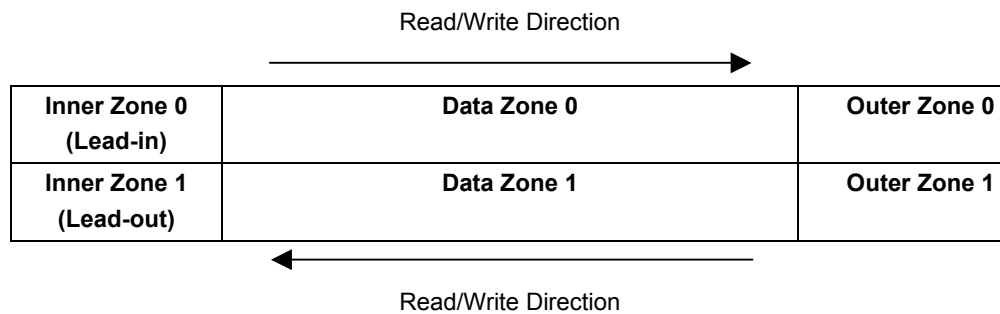
Figure 80 — Primary Zones of a Dual Layer BD-R
