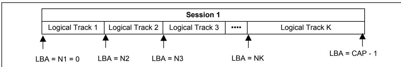
Figure 92 — Status of BD-R Disc Multiple RESERVE TRACK Commands
