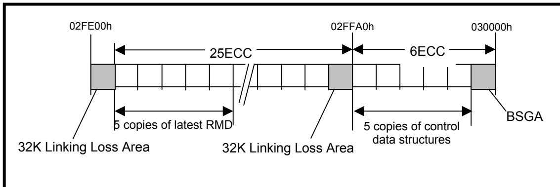
Figure 32 — Structure of Extra Border Zone
