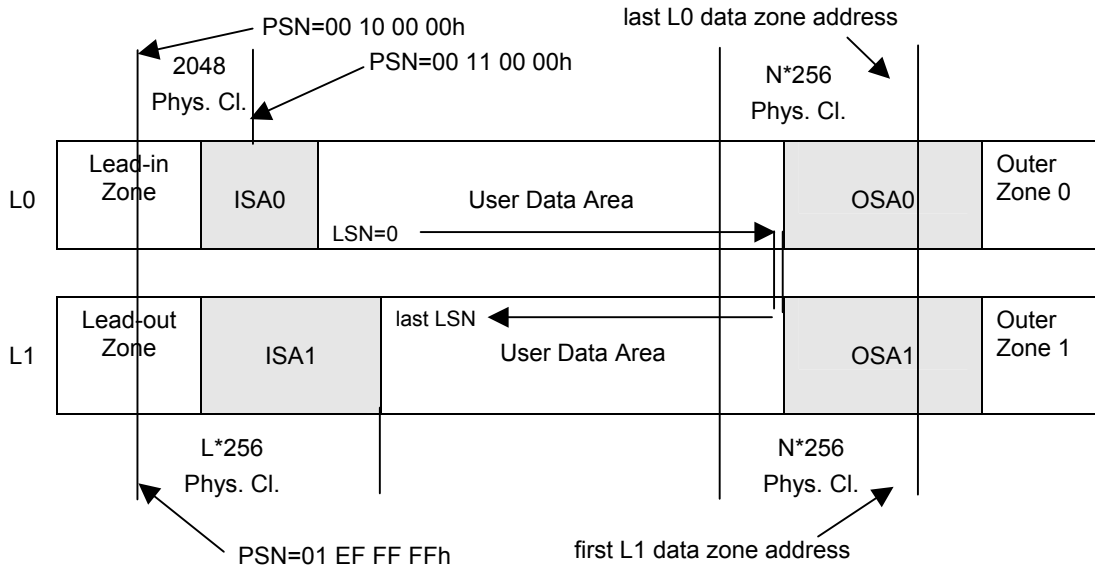
Figure 103 — Layout of Dual Layer BD-RE Disc
