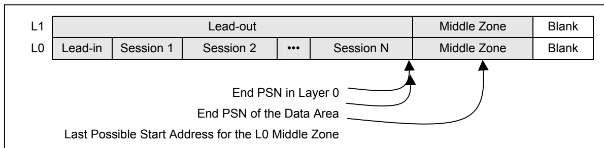
Figure 51 — Preferred Single Layer Recording
