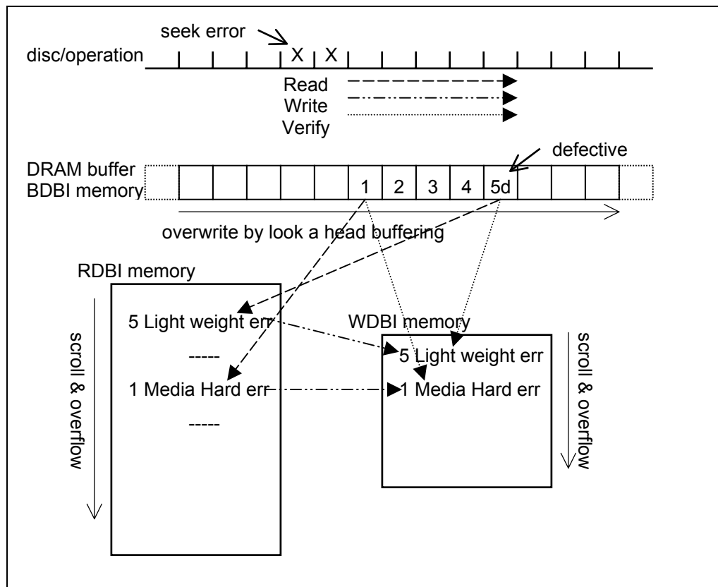
Figure 110 — Example of DBI memory blocks
