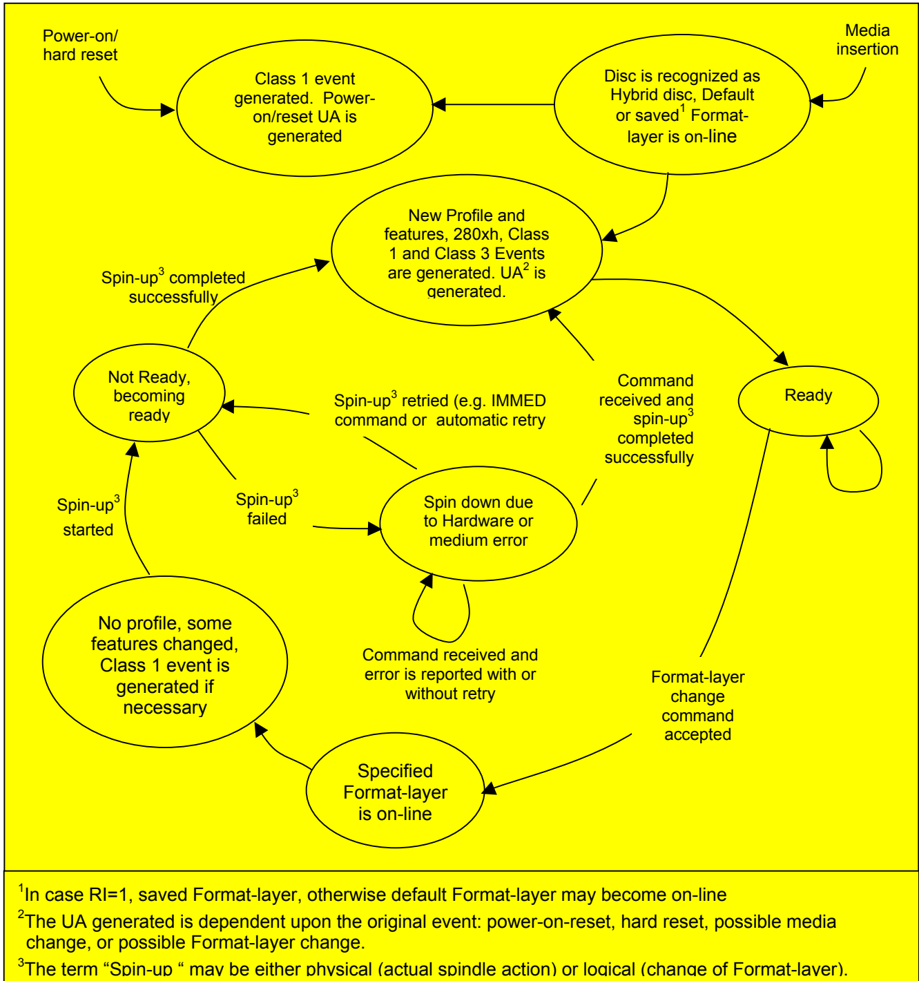
Figure 125 — State diagram of Format-layer changing
