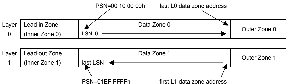
Figure 77 — Layout of Dual Layer BD-ROM Information Zone
