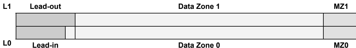
Figure 65 — Finalization part of the format process
