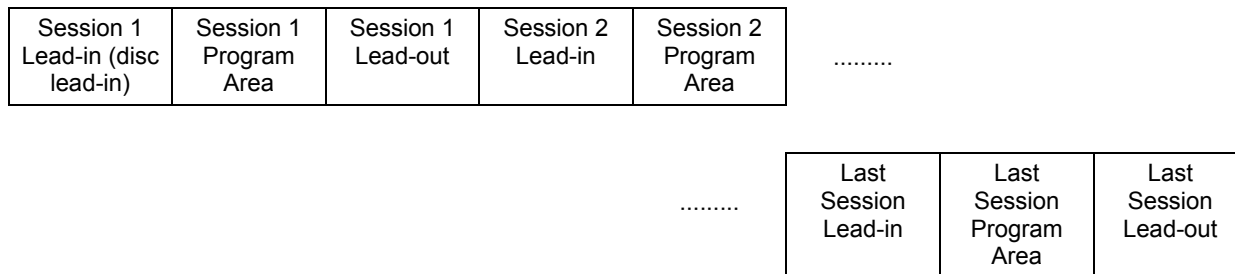
Figure 10 — Multi-Session Recorded Disc
