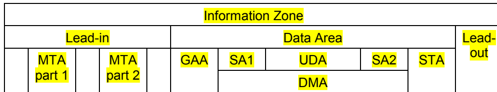
Figure 35 – MRW Mapping onto DVD+RW, General
