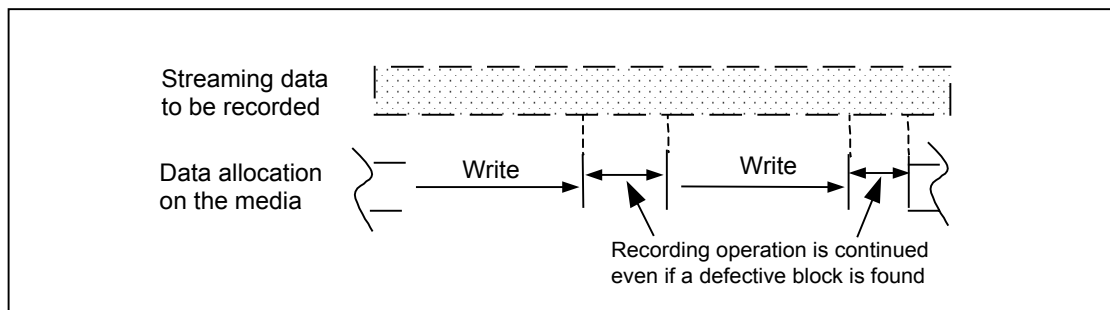
Figure 39 – An example of data allocation on the Stream recording operation
