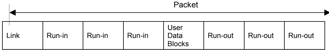
Figure 18 – Packet Layout
