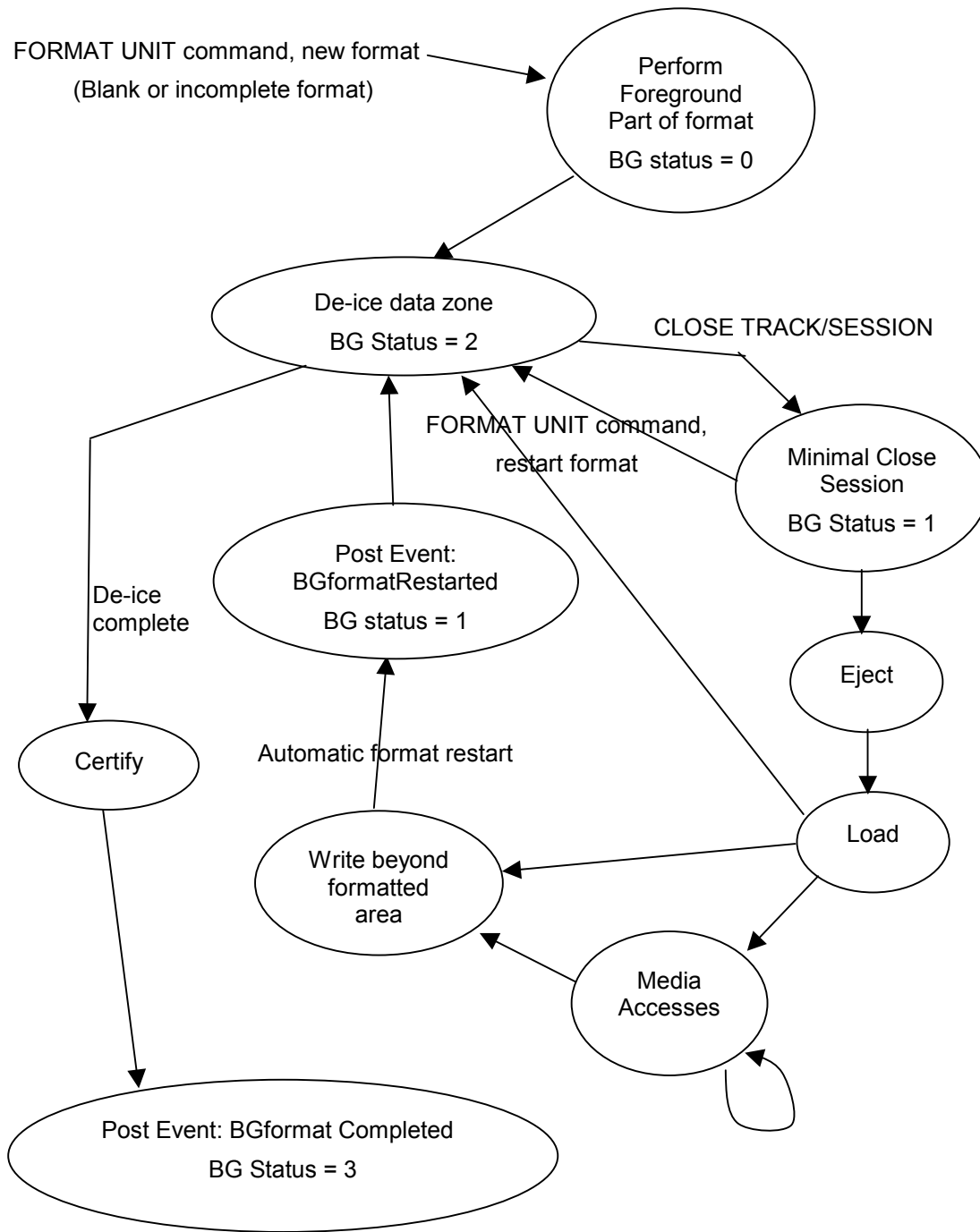
Figure 40 – Background Process Flow
