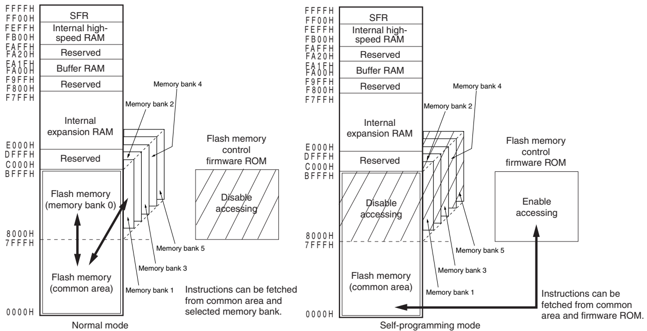
Figure 26-15. Operation Mode and Memory Map for Self-Programming (μPD78F0537)
