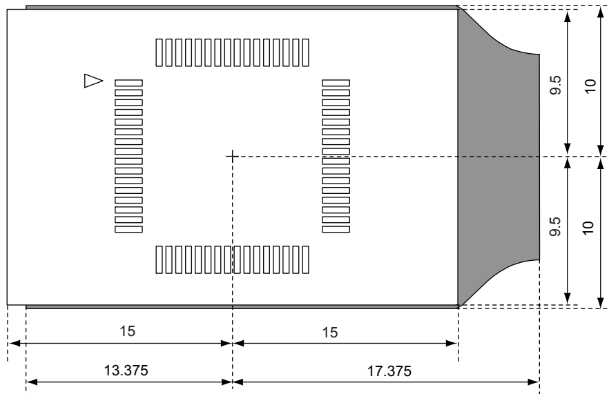
Figure B-2. For 64-Pin GA Package
