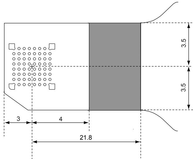
Figure B-1. For 64-Pin FC Package
