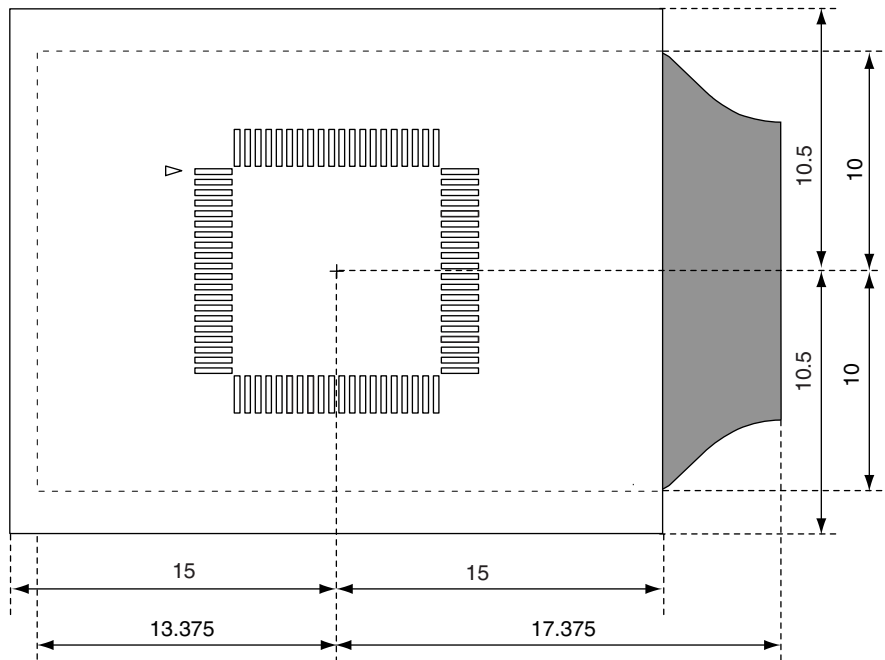
Figure B-3. For 64-Pin GB Package
