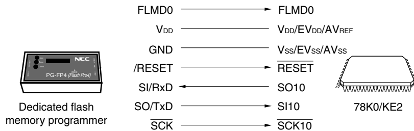
Figure 26-6. Communication with Dedicated Flash Memory Programmer (CS10)
