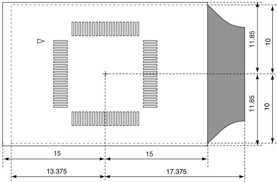
Figure B-4. For 64-Pin GC Package
