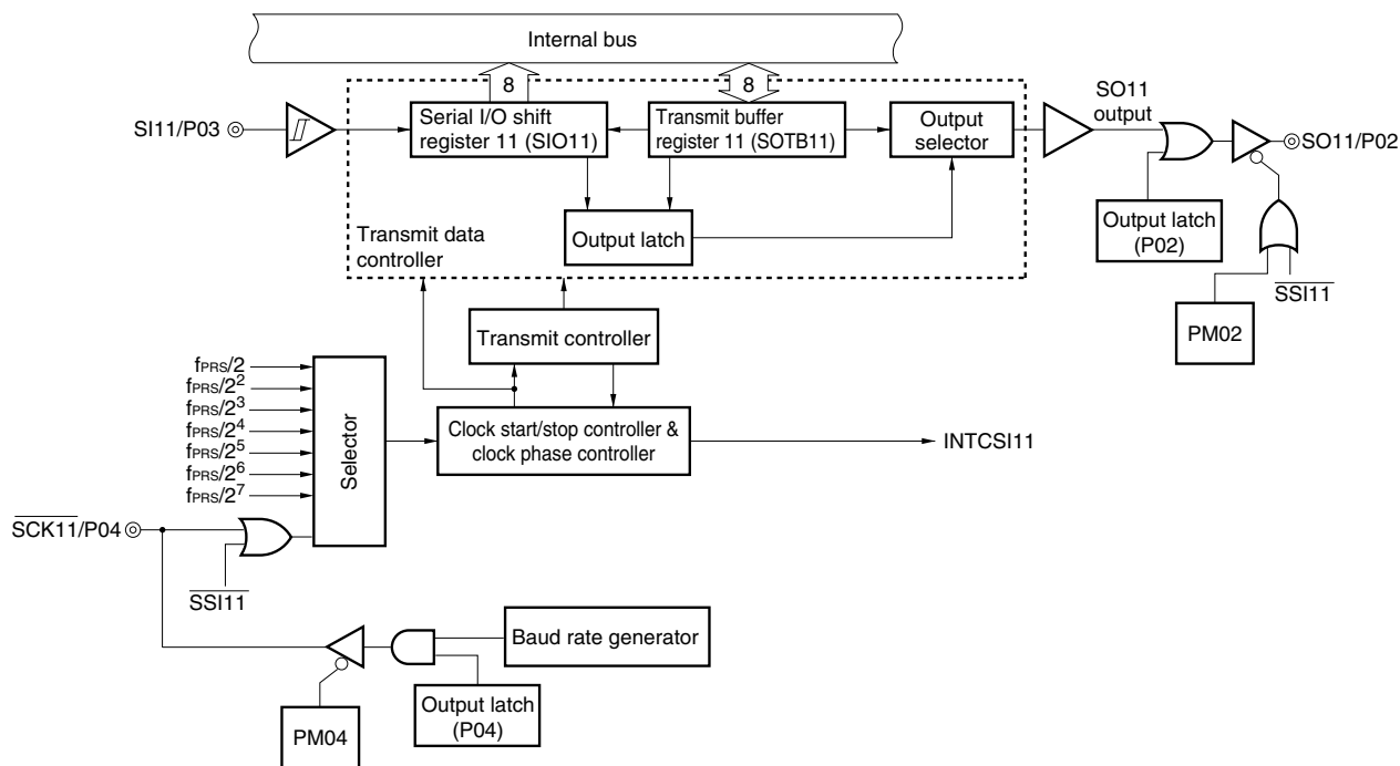
Figure 16-2. Block Diagram of Serial Interface CSI11 (Available only in the \mu PD78F0534, 78F0535, 78F0536, 78F0537, 78F0537D)
