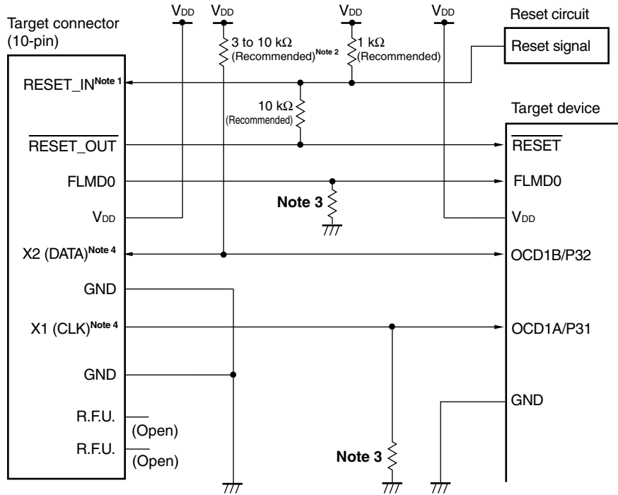
Figure 27-2. Connection Example of QB-78K0MINI or QB-MINI2 and \mu PD78F0537D (When OCD1A/P31 and OCD1B/P32 Are Used)
