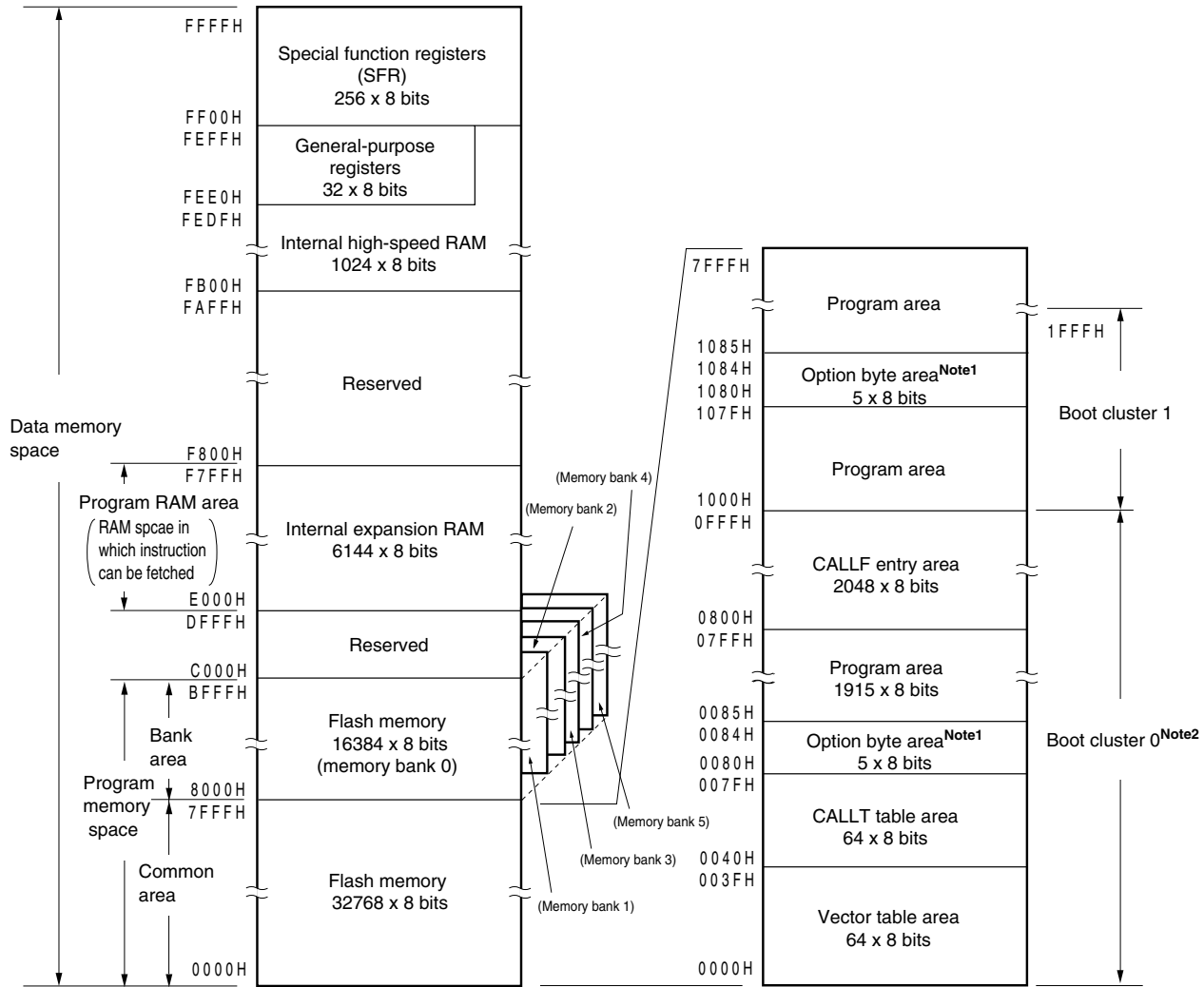
Figure 3-7. Memory Map ( \mu PD78F0537)
