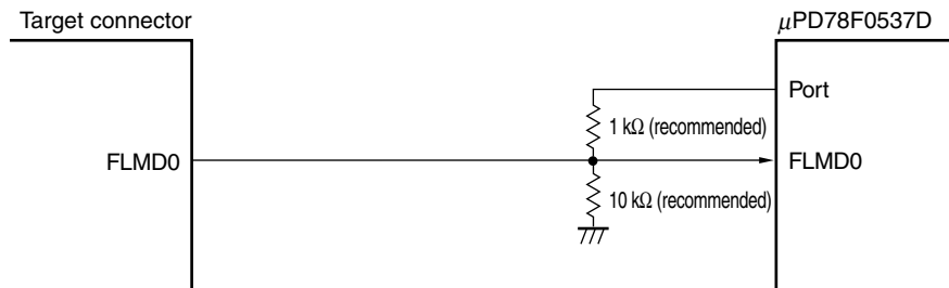
Figure 27-3. Connection of FLMD0 Pin for Self Programming by Means of On-Chip Debugging
