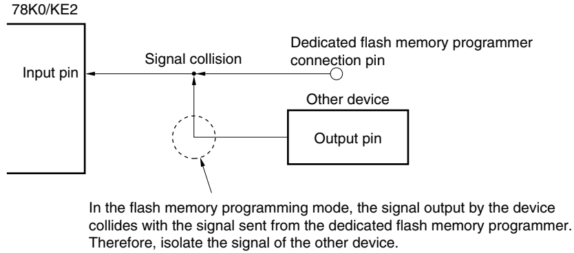
Figure 26-9. Signal Collision (Input Pin of Serial Interface)
