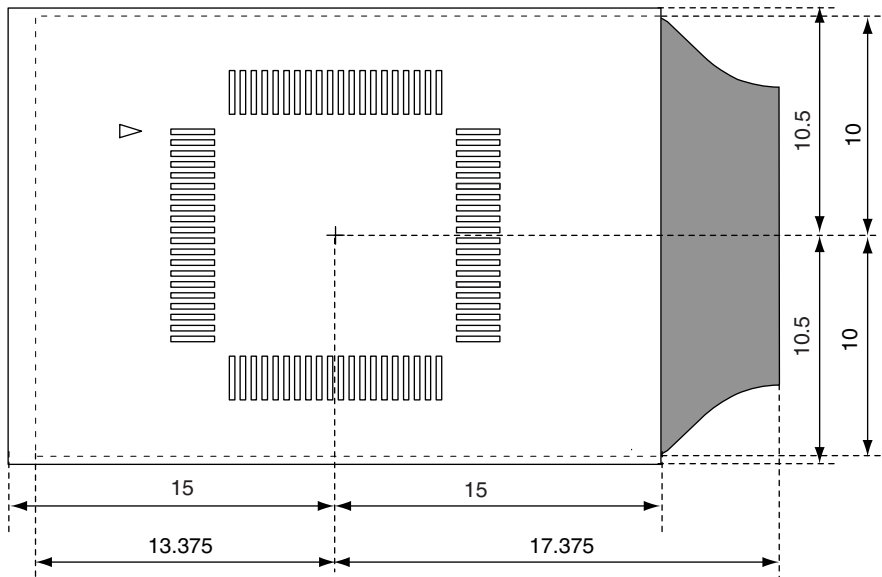
Figure B-5. For 64-Pin GK Package
