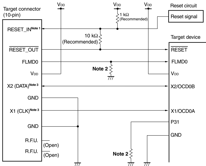
Figure 27-1. Connection Example of QB-78K0MINI or QB-MINI2 and \mu PD78F0537D (When OCD0A/X1 and OCD0B/X2 Are Used)
