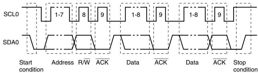
Figure 17-12. I 2 C Bus Serial Data Transfer Timing
