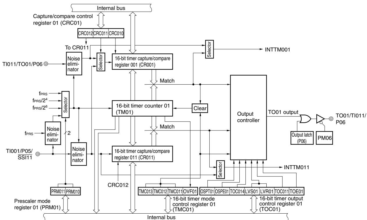
Figure 7-2. Block Diagram of 16-Bit Timer/Event Counter 01 (Available only in the \mu PD78F0534, 78F0535, 78F0536, 78F0537, and 78F0537D)
